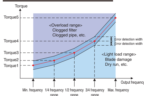
Load characteristic measurement function
